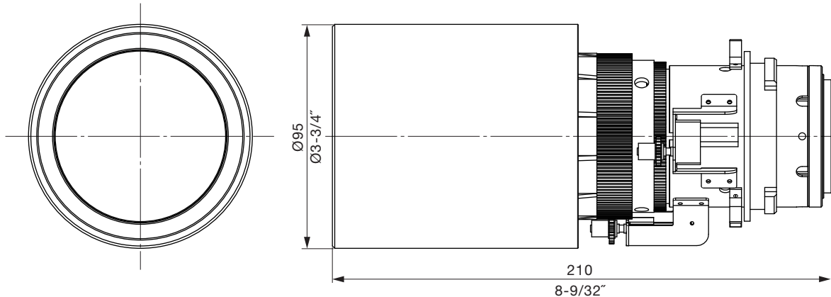
Illustration shows the lens attached to the PT-DZ6710/DZ6710/DZ6700/DZ6700L/DW6300S/DW6300LS/DW6300K/DW6300LK/D6000S/D6000LS/D6000K/D6000LK.
