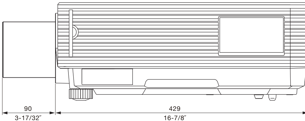
The illustration shows the lens attached to the PT-D4000.
