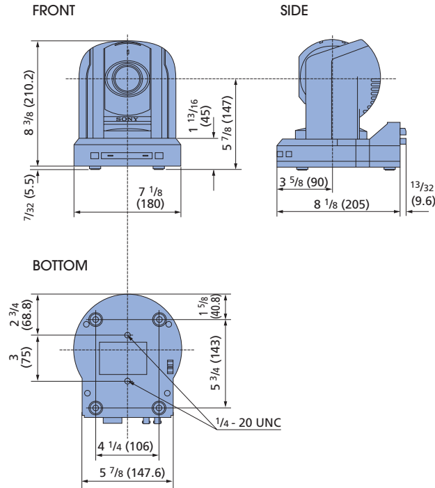
BRC-300/BRC-300P
