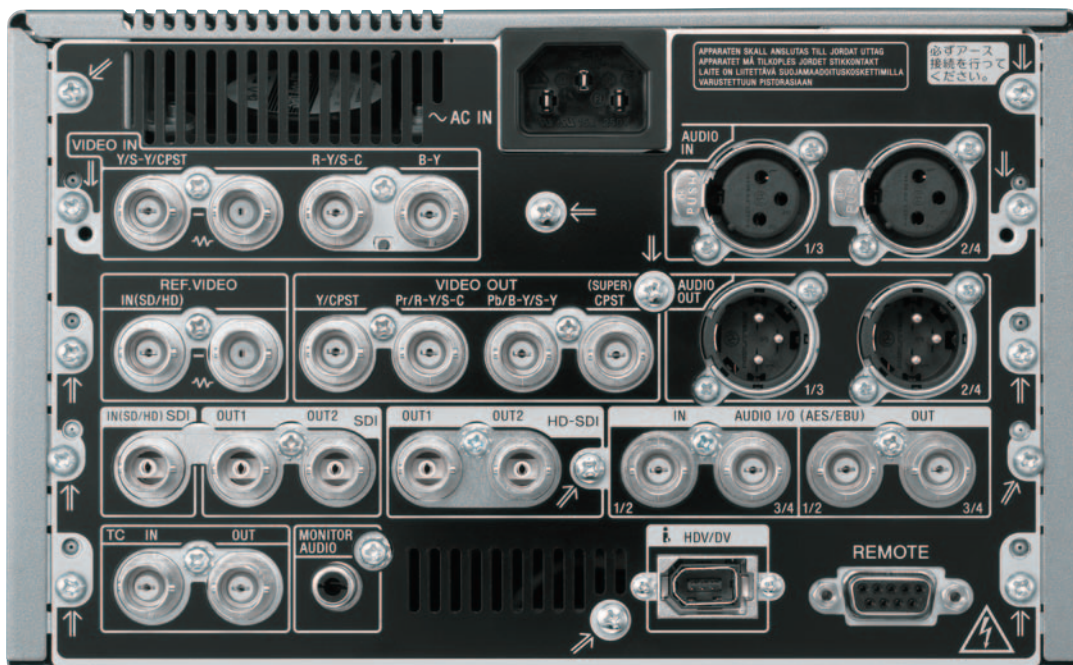
Rear panel of the HVR-1500A (with the optional HVBK-1505 board)
